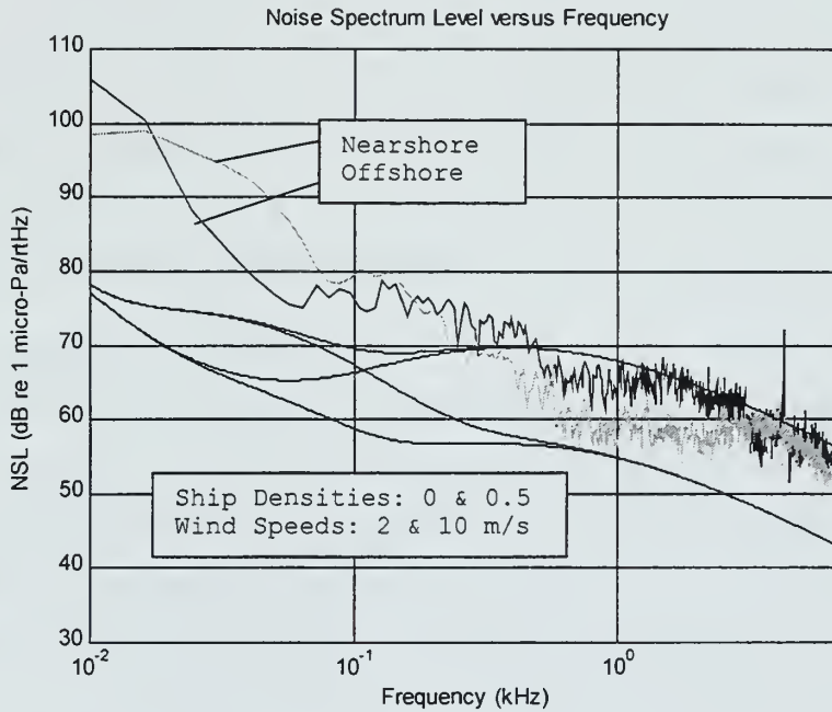
Figure 4.7. Observed 12-Hz-band-average NSL versus frequency for the Nearshore and Offshore locations. The estimated NSLs are for D=0 and 0.5, and w=2 and 10 m/s. Total broadband (0-6.4 kHz) NLs are 113 dB and 116 dB re 1 \mu Pa for Nearshore and Offshore, respectively.
